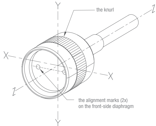
The principal axes of the sensor
